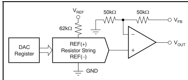
Figure 45. DAC8550 Architecture
