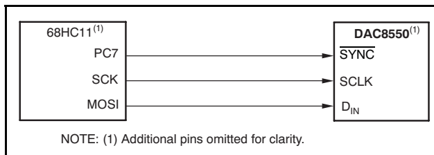
Figure 52. DAC8550 to 68HC11 Interface
