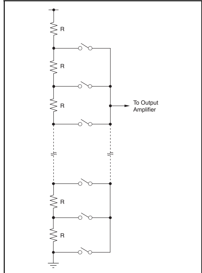
Figure 46. Resistor String
