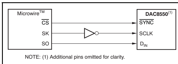
Figure 51. DAC8550 to Microwire Interface
